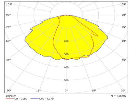
Luminance Distribution
