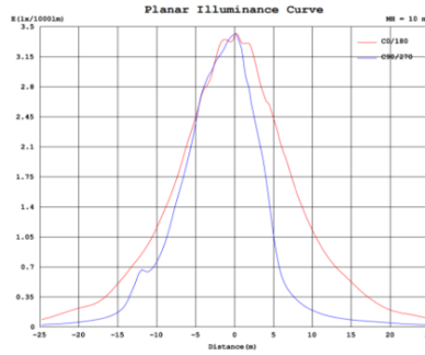
Illumination Curve
